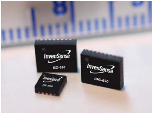
Figure 2: InvenSense™ integrated 6-axis motion processing solution with 7x7mm total area
