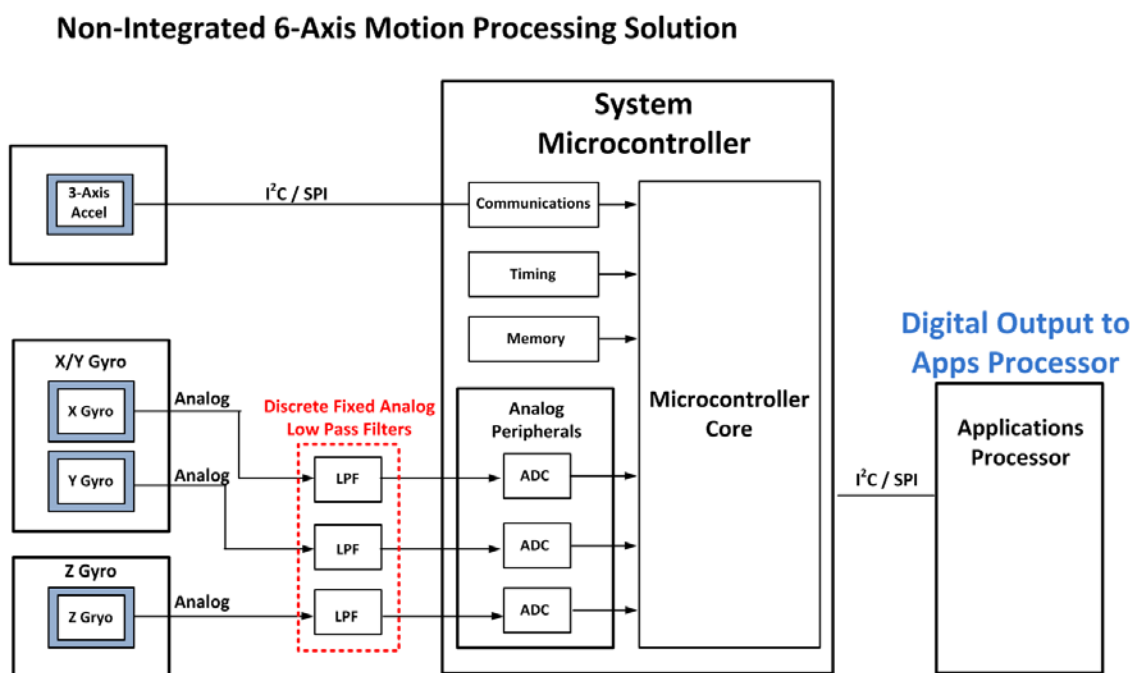
Figure 4: Non-integrated solutions using disparate motion sensors requires signal conditioning with discrete fixed functionality.
