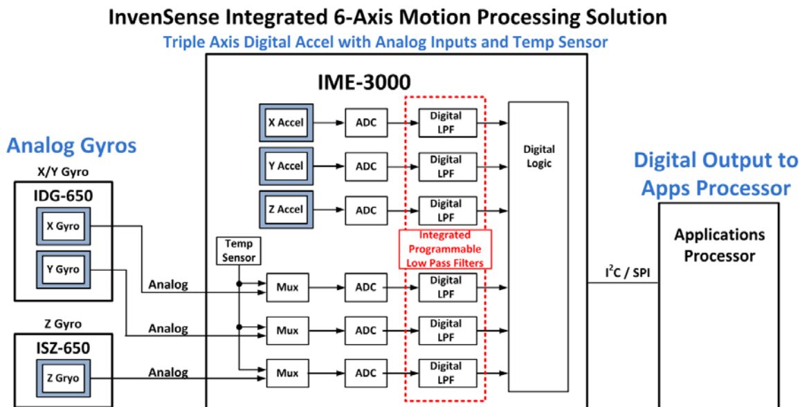
Figure 5: An integrated motion processing solution with programmable signal conditioning eliminates the need for fixed frequency external low pass filters.
