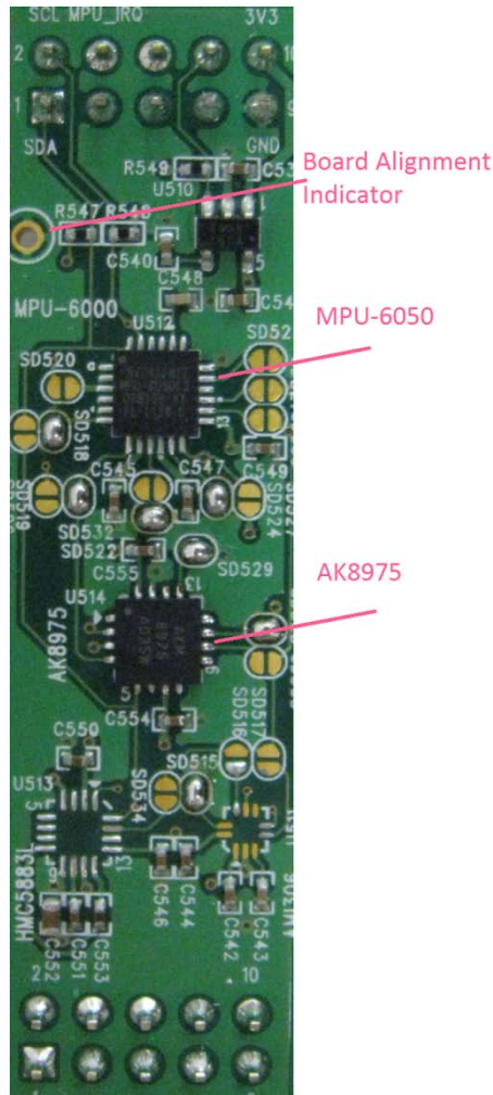
Figure 3-1. Sensor arrangement
